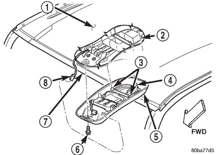
Fig. 5 Overhead Console Remove/Install
