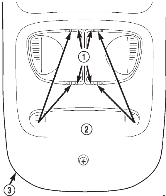
Fig. 4 Overhead Console Reading and Courtesy Lamp Lens Remove/Install
