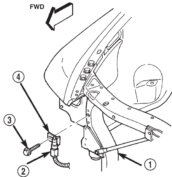
Fig. 10 Ambient Temperature Sensor Remove/Install
